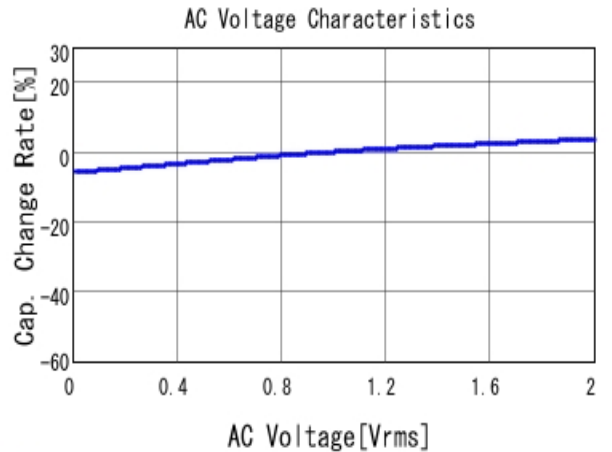
GCM32DC72A475KE02 C-AC Voltage capchange, DCOV, 25.0d
