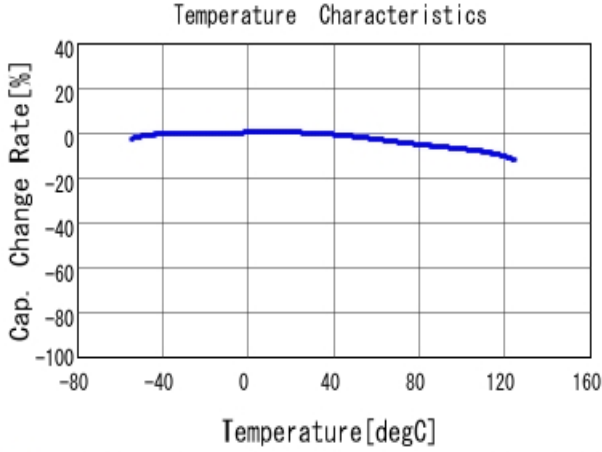
GCM32DC72A475KE02 C-Temp. capchange, DC0.0V, AC1.0V rm
