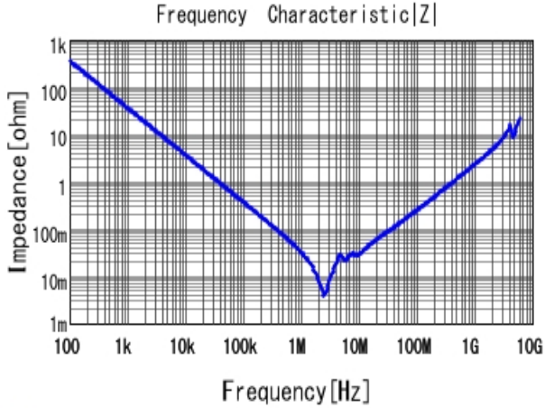
GCM32DC72A475KE02 |Z| DCOV, 25degC
