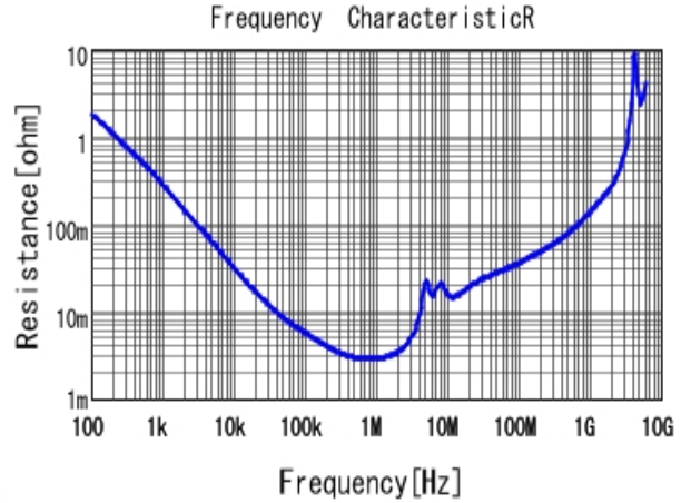
GCM32DC72A475KE02 R DCOV, 25degC
