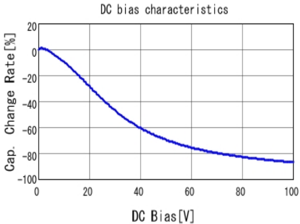
GCM32DC72A475KE02 C-DC bias capchange, 25.0degC, AC1.
