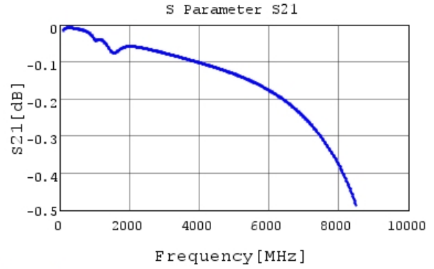
GCM1555C1H331JA16 S21 DCOV, 25degC
