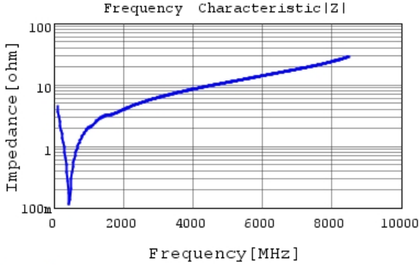
GCM1555C1H331JA16 |Z| DC0V, 25degC
