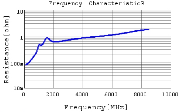
GCM1555C1H331JA16 R DC0V, 25degC
