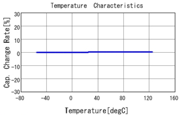
GJM0335C1E1R4BB01 C-Temp. capchange, DC0V, AC1Vrms
