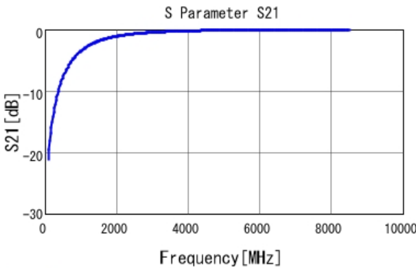
GJM0335C1E1R4BB01 S21 DC0V, 25degC
