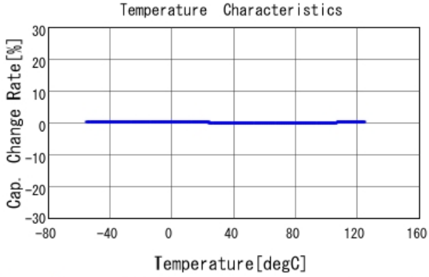
GRM2165C1H183GA01 C-Temp. capchange, DCOV, AC1Vrms
