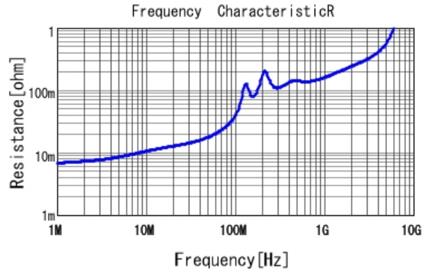
GRM2165C1H183GA01 R DCOV, 25degC
