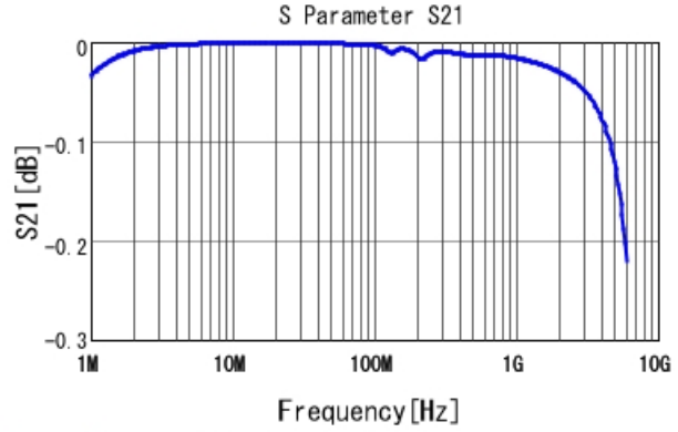
GRM2165C1H183GA01 S21 DCOV, 25degC
