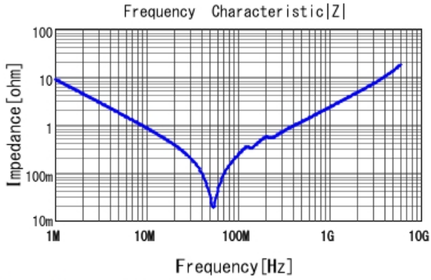
GRM2165C1H183GA01 |Z| DCOV, 25degC
