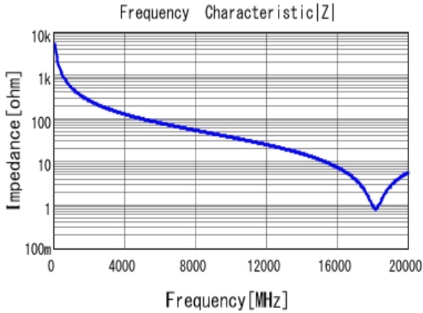
■ GRM0225C1ER30WA03 |Z| DCOV, 25degC
