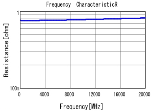
■ GRM0225C1ER30WA03 R DCOV, 25degC
