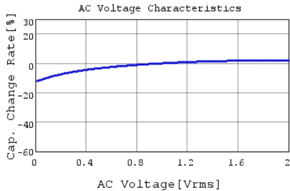
GRM033R61C473KE84 C-AC Voltage capchange, Dc
