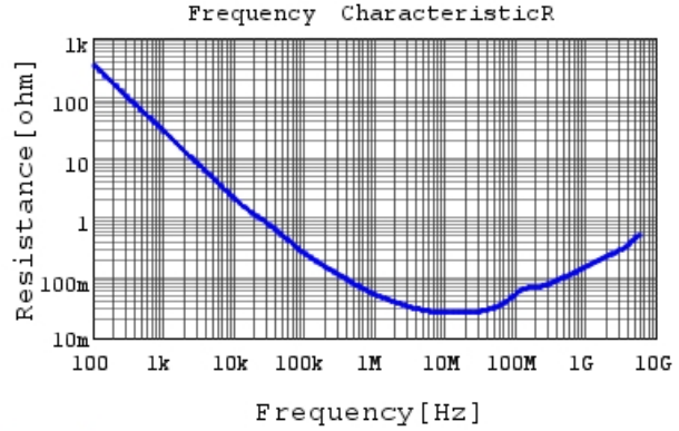
GRM033R61C473KE84 R DCOV, 25degC
