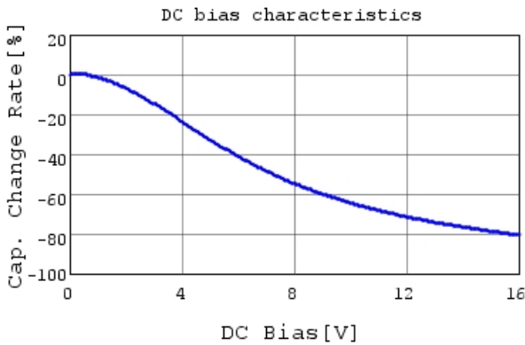
GRM033R61C473KE84 C-DC bias capchange, 25.0c
