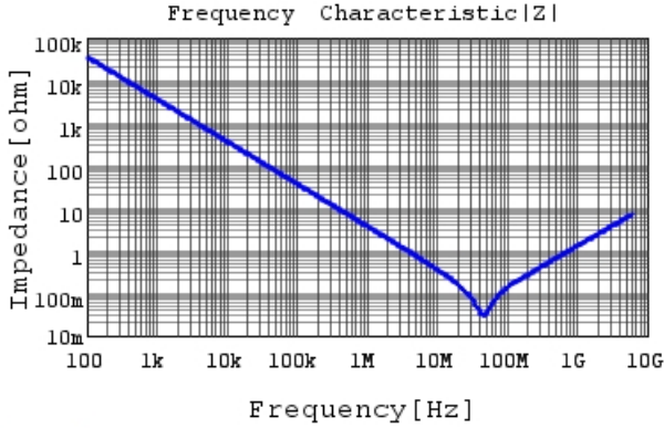
GRM033R61C473KE84 |Z| DCOV, 25degC
