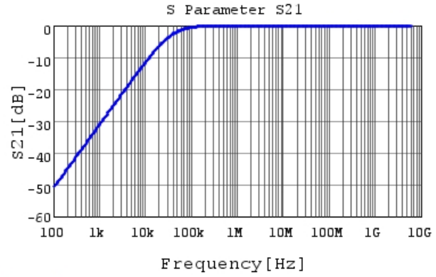
GRM033R61C473KE84 S21 DC0V, 25degC
