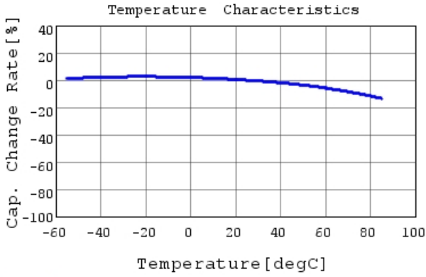
GRM033R61C473KE84 C-Temp. capchange, DC0.0V,
