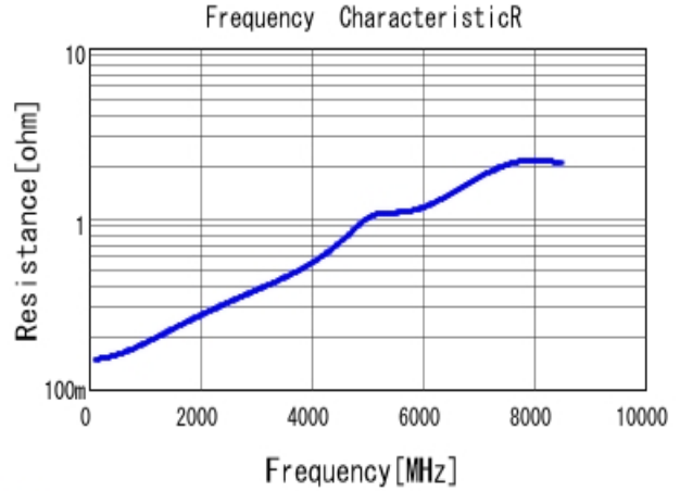
■ GRM0332C1H240JA01 R DCOV, 20degC
