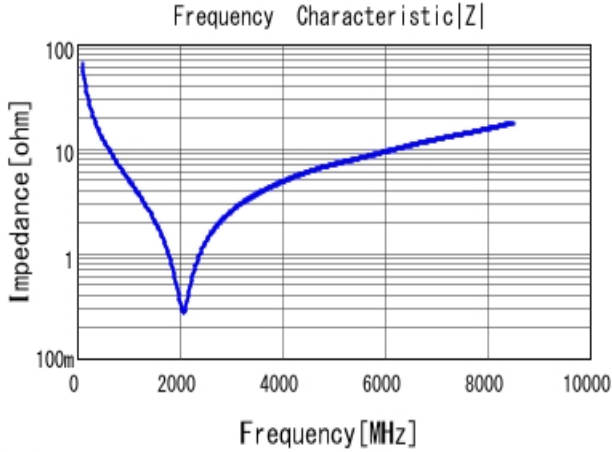
■ GRM0332C1H240JA01 |Z| DCOV, 20degC
