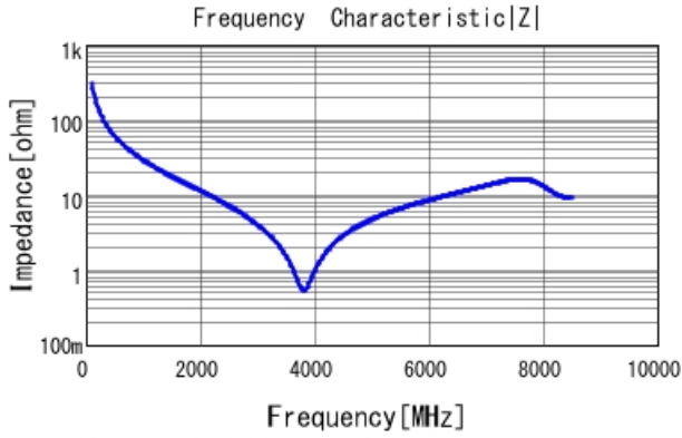
GRM1555C1H5R1BA01 |Z| DCOV, 25degC
