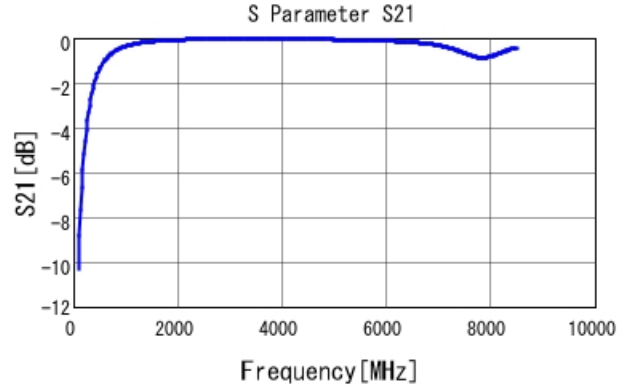
GRM1555C1H5R1BA01 S21 DC0V, 25degC
