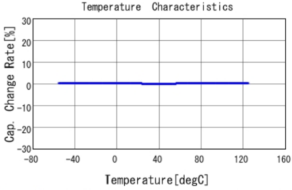
GRM1555C1H5R1BA01 C-Temp. capchange, DC0V, AC1Vrms
