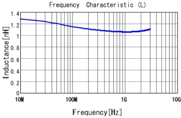
LQP03TG1N1C02 L
