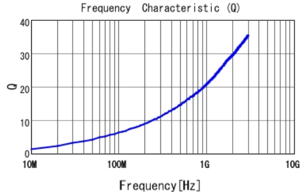
LQP03TG1N1C02 Q
