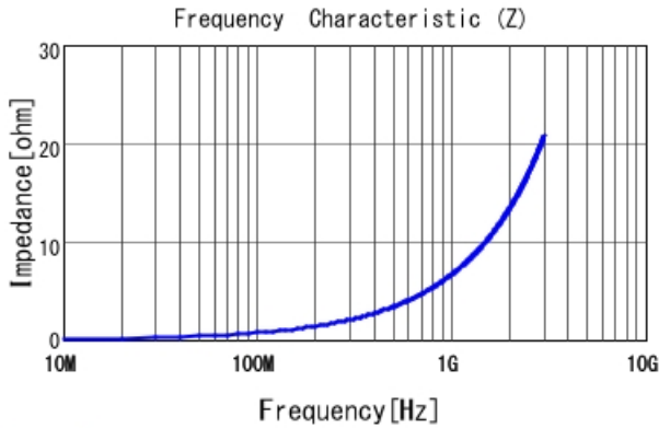
LQP03TG1N1C02 |Z|
