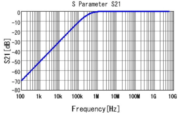
GRM155R61H472KA01 S21 DC0V, 25degC
