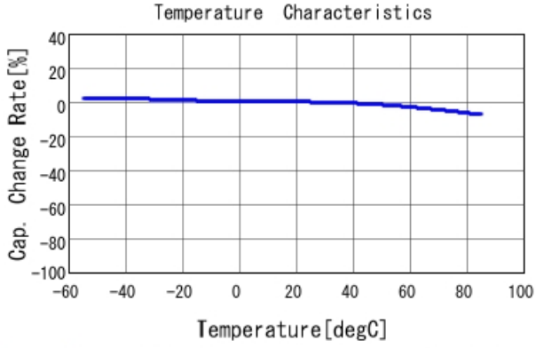
GRM155R61H472KA01 C-Temp. capchange, DC0.0V, AC1.C
