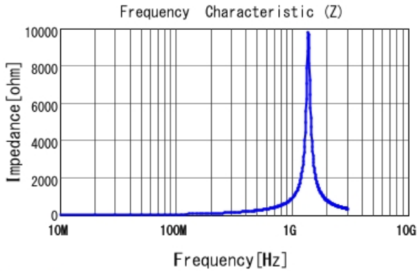
LQP03TN75NH02 |Z|
