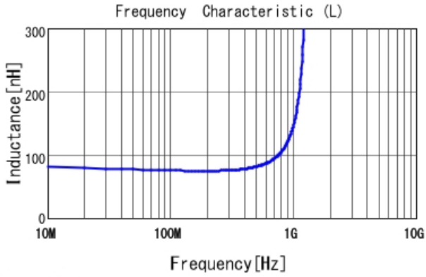
LQP03TN75NH02 L
