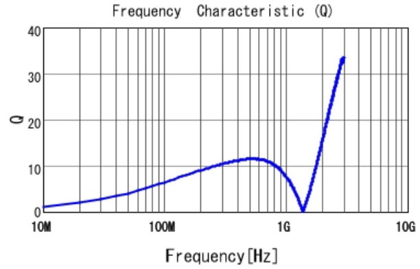
LQP03TN75NH02 Q
