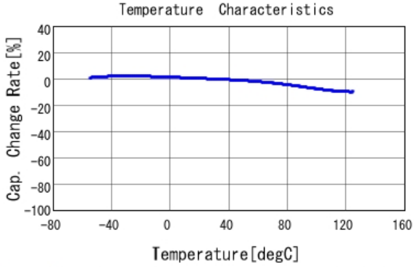
GRM31MR72A474KA35 C-Temp. capchange, DC0.0V, AC1.C
