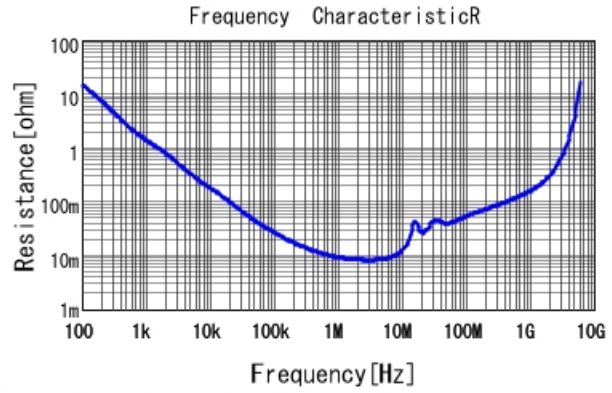
GRM31MR72A474KA35 R DCOV, 25degC
