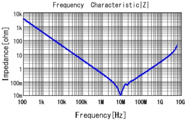
GRM31MR72A474KA35 |Z| DCOV, 25degC
