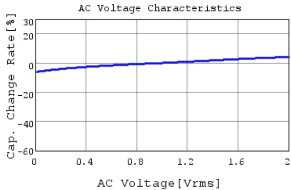
■ LLL185R71A224MA01 C-AC Voltage capchange, DC
