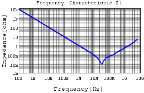
■ LLL185R71A224MA01 |Z| DCOV, 25degC
