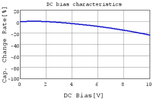
■ LLL185R71A224MA01 C-DC bias capchange, 25.0c
