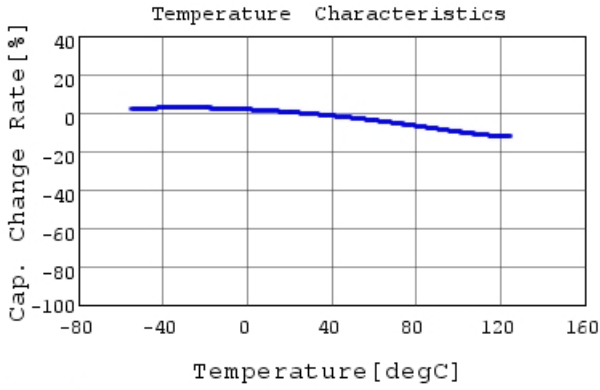
LLL185R71A224MA01 C-Temp. capchange, DC0.0V,
