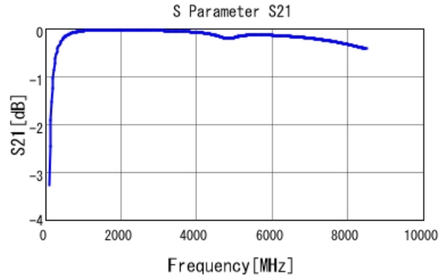
GCM1555G1H150JA16 S21 DCOV, 25degC
