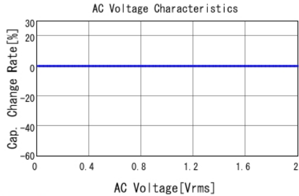
GCM1555G1H150JA16 C-AC Voltage capchange, DCOV, 25
