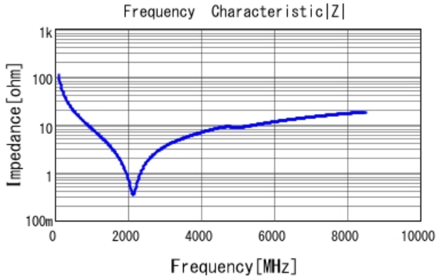
GCM1555G1H150JA16 |Z| DCOV, 25degC
