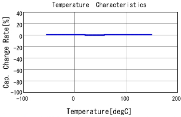
GCM1555G1H150JA16 C-Temp. capchange, DCOV, AC1Vrms
