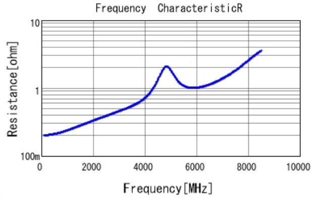
GCM1555G1H150JA16 R DCOV, 25degC
