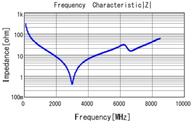
GCM1885C2A5R6CA16 |Z| DCOV, 25degC
