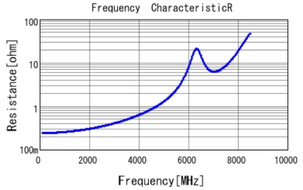
GCM1885C2A5R6CA16 R DCOV, 25degC
