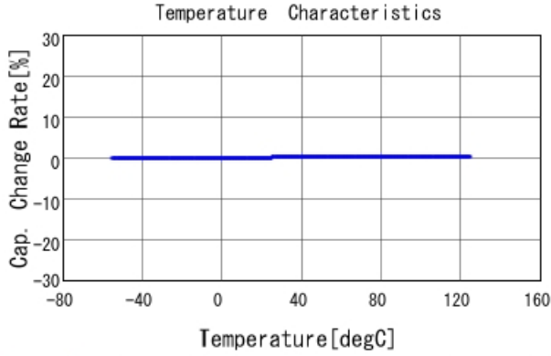
GCM1885C2A5R6CA16 C-Temp. capchange, DC0V, AC1Vrms
