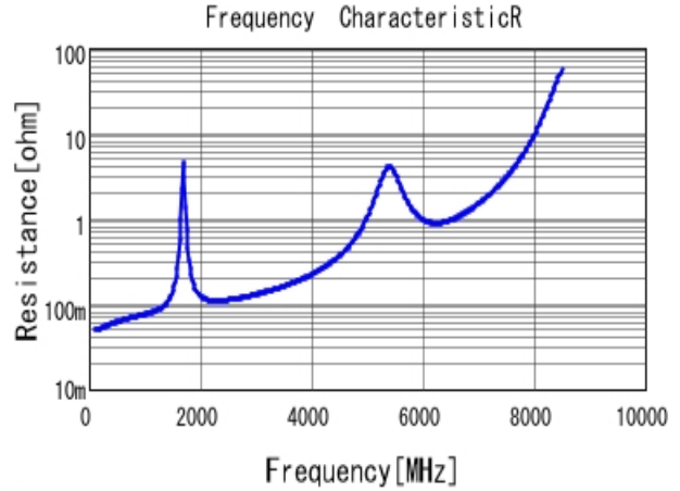
■ GQM1885C1H620GB01 R DCOV, 25degC
