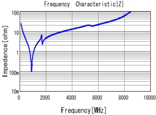
■ GQM1885C1H620GB01 |Z| DCOV, 25degC
