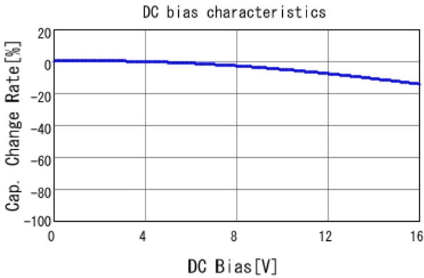
GRM31MR71C105MA01 C-DC bias capchange, 25.0degC, A
