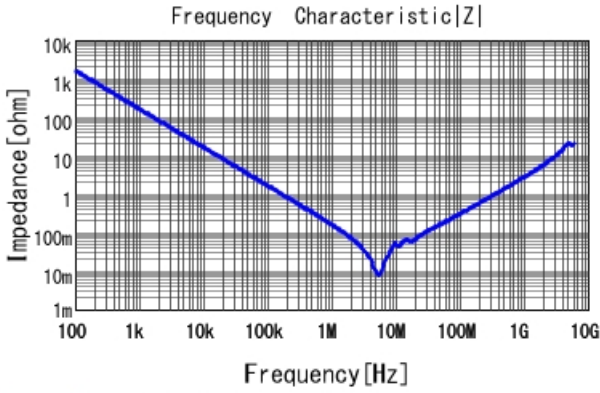
GRM31MR71C105MA01 |Z| DCOV, 25degC
