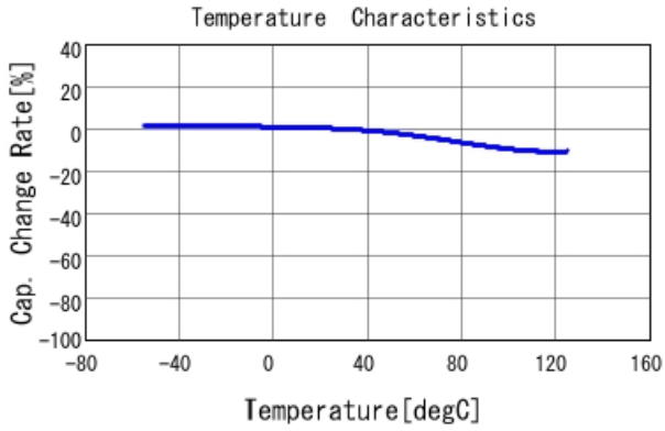
GRM31MR71C105MA01 C-Temp. capchange, DC0.0V, AC1.C
