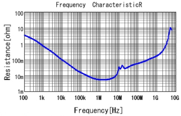
GRM31MR71C105MA01 R DCOV, 25degC
