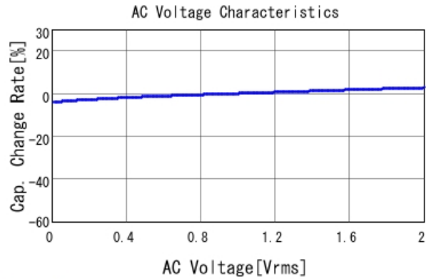
GRM31MR71C105MA01 C-AC Voltage capchange, DCOV, 25
