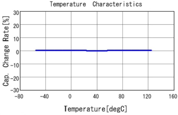
GRM1555C2A6R7BA01 C-Temp. capchange, DCOV, AC1Vrms
