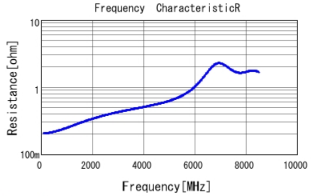
GRM1555C2A6R7BA01 R DCOV, 25degC
