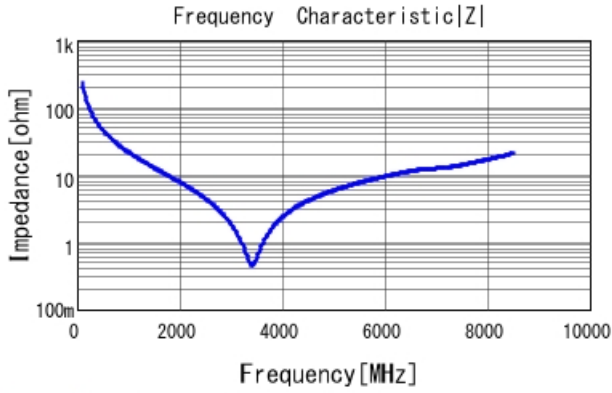
GRM1555C2A6R7BA01 |Z| DCOV, 25degC
