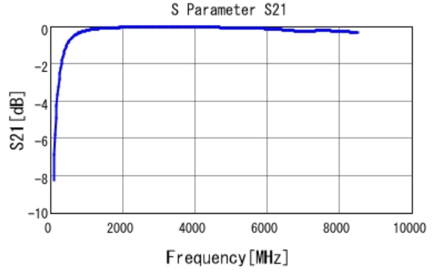
GRM1555C2A6R7BA01 S21 DCOV, 25degC
