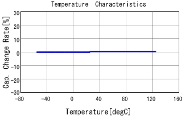
GJM0335C1E7R0BB01 C-Temp. capchange, DC0V, AC1Vrms
