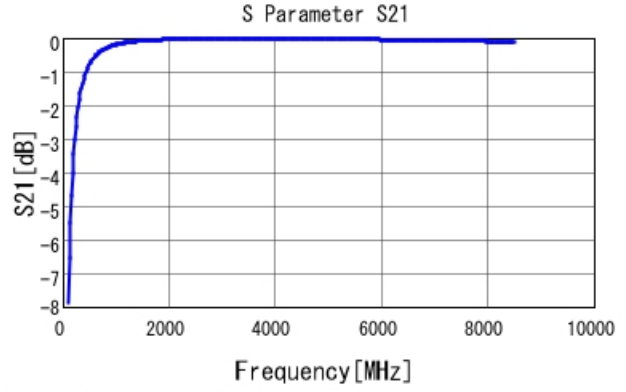
GJM0335C1E7R0BB01 S21 DC0V, 25degC
