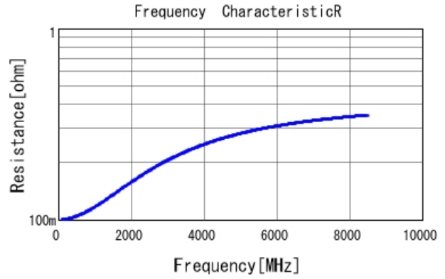
GJM0335C1E7R0BB01 R DCOV, 25degC
