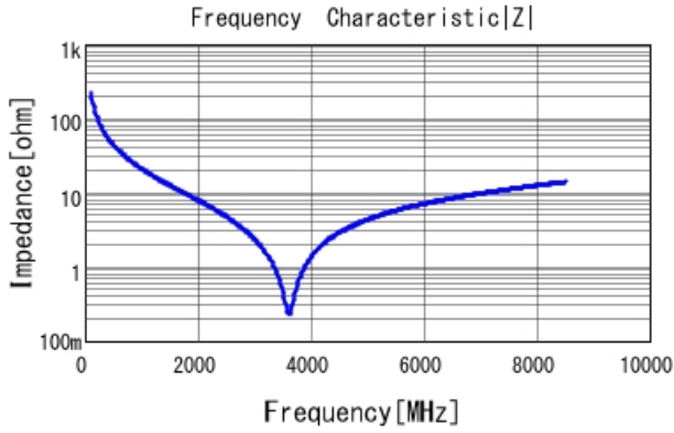
GJM0335C1E7R0BB01 |Z| DCOV, 25degC
