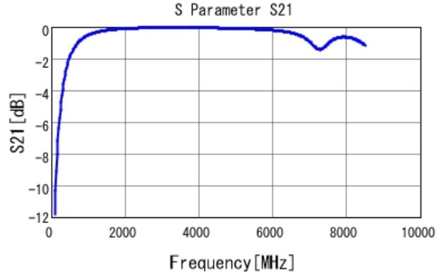
GRM1885C1H4R2WA01 S21 DCOV, 25degC
