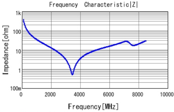
GRM1885C1H4R2WA01 |Z| DCOV, 25degC
