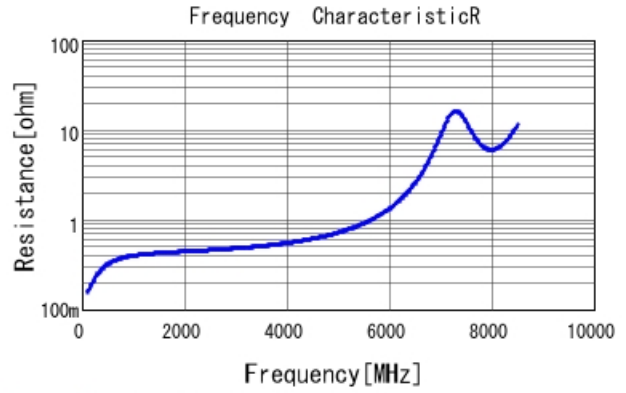
GRM1885C1H4R2WA01 R DCOV, 25degC
