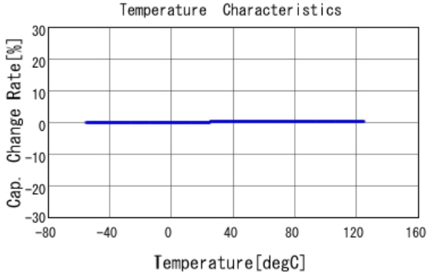
GRM1885C1H4R2WA01 C-Temp. capchange, DCOV, AC1Vrms
