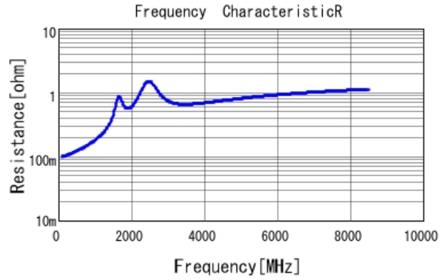
GCM1555G1H121JA16 R DCOV, 25degC
