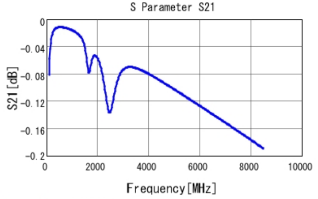
GCM1555G1H121JA16 S21 DCOV, 25degC
