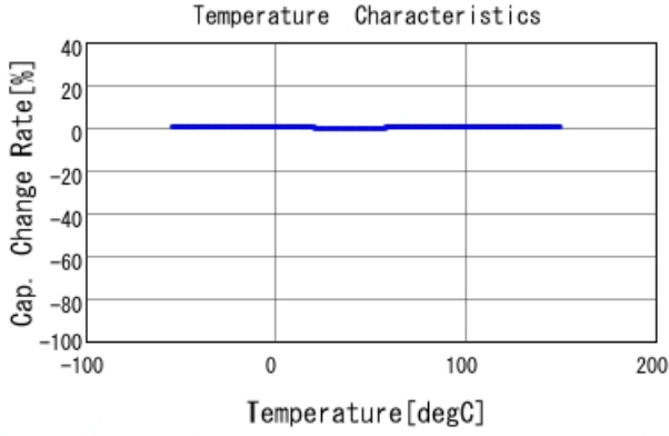
GCM1555G1H121JA16 C-Temp. capchange, DCOV, AC1Vrms
