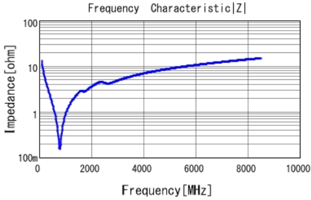
GCM1555G1H121JA16 |Z| DCOV, 25degC
