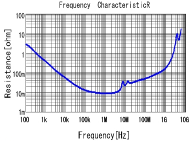
■ GRJ32DR72A225KE11 R DCOV, 25degC
