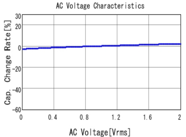
■ GRJ32DR72A225KE11 C-AC Voltage capchange, DCOV, 25.0d
