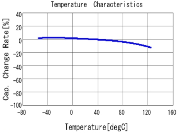
■ GRJ32DR72A225KE11 C-Temp. capchange, DC0.0V, AC1.0V r m
