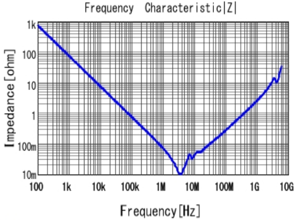
■ GRJ32DR72A225KE11 |Z| DCOV, 25degC
