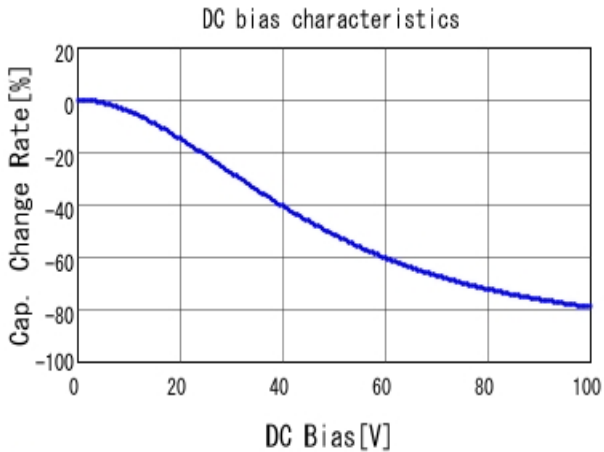
■ GRJ32DR72A225KE11 C-DC bias capchange, 25.0degC, AC1.
