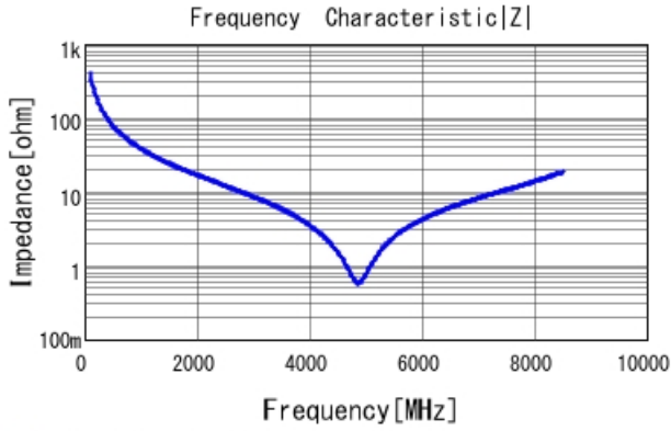
■ GRM0335C2A4R0CA01 |Z| DCOV, 25degC
