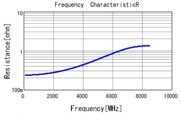
■ GRM0335C2A4R0CA01 R DCOV, 25degC
