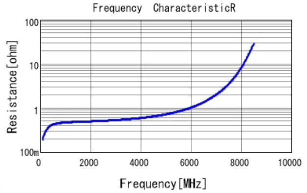
GRM1885C2A3R2CA01 R DCOV, 25degC
