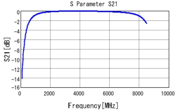
GRM1885C2A3R2CA01 S21 DCOV, 25degC
