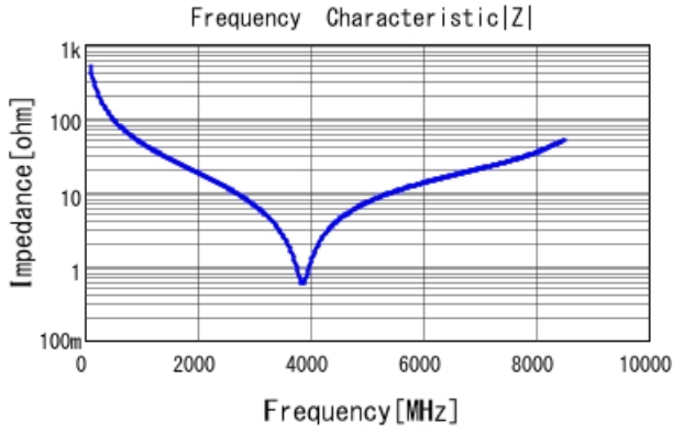
GRM1885C2A3R2CA01 |Z| DCOV, 25degC
