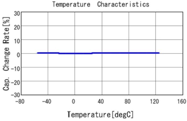
GQM2195C2E390JB12 C-Temp. capchange, DCOV, AC1Vrms
