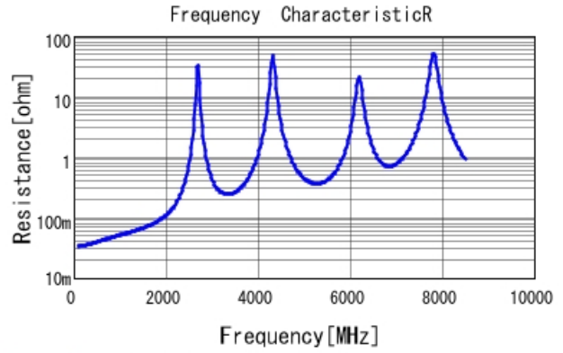
GQM2195C2E390JB12 R DCOV, 25degC
