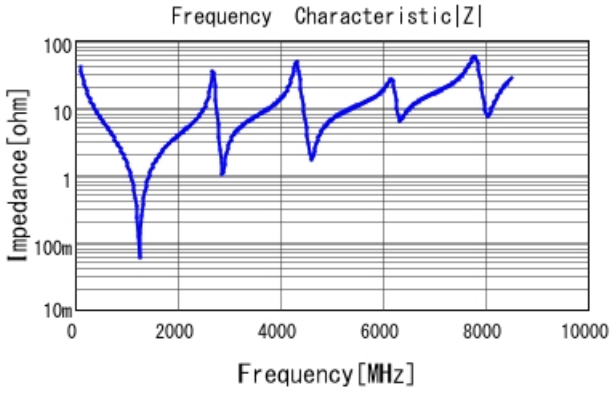
GQM2195C2E390JB12 |Z| DCOV, 25degC
