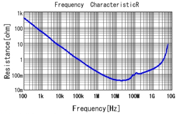
■ GCJ188R92A473MA01 R DCOV, 25degC
