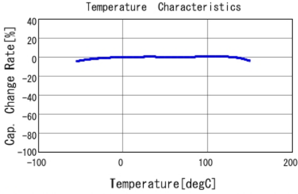
■ GCJ188R92A473MA01 C-Temp. capchange, DCO. 0V, AC1. 0Vrm
