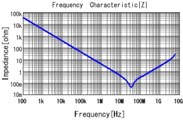
■ GCJ188R92A473MA01 |Z| DCOV, 25degC
