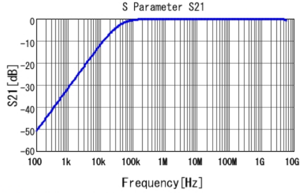
■ GCJ188R92A473MA01 S21 DCOV, 25degC
