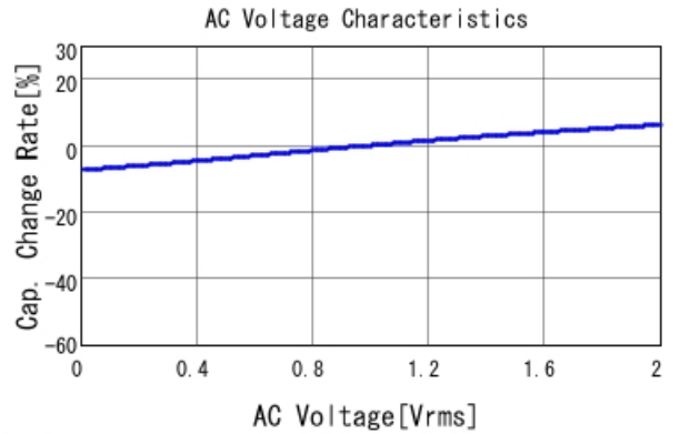
■ GCJ188R92A473MA01 C-AC Voltage capchange, DCOV, 25.0d
