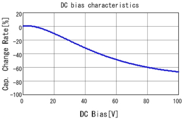
■ GCJ188R92A473MA01 C-DC bias capchange, 25.0degC, AC1.
