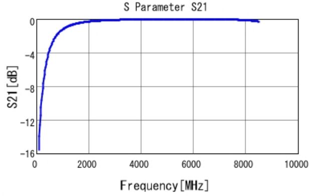
GJM0335C1E2R7WB01 S21 DC0V, 25degC
