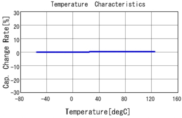
GJM0335C1E2R7WB01 C-Temp. capchange, DC0V, AC1Vrms
