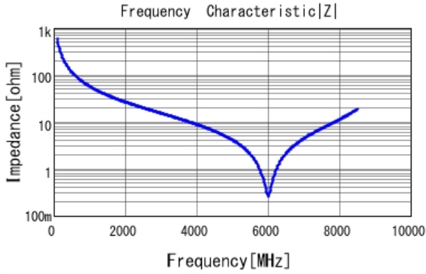
GJM0335C1E2R7WB01 |Z| DCOV, 25degC
