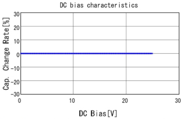
GJM0335C1E2R7WB01 C-DC bias capchange, 25.0degC, A
