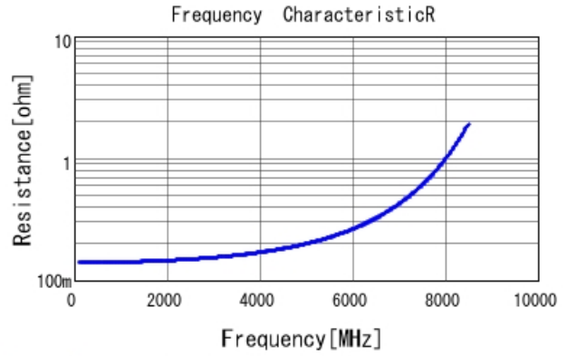
GJM0335C1E2R7WB01 R DCOV, 25degC
