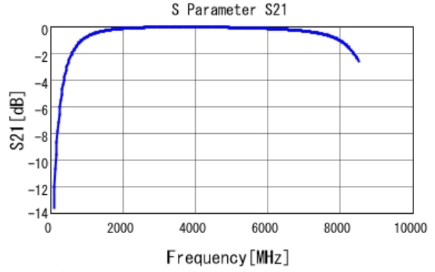
GRM1885C1H3R4CA01 S21 DCOV, 25degC
