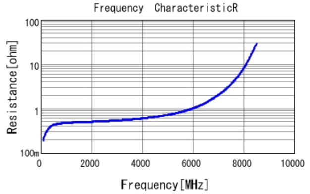
GRM1885C1H3R4CA01 R DCOV, 25degC
