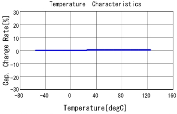
GRM1885C1H3R4CA01 C-Temp. capchange, DCOV, AC1Vrms
