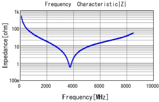
GRM1885C1H3R4CA01 |Z| DCOV, 25degC
