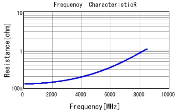
GJM1555C1H3R4CB01 R DCOV, 25degC
