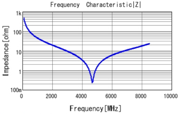
GJM1555C1H3R4CB01 |Z| DCOV, 25degC
