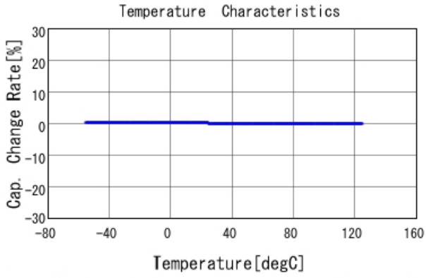
GRM0335C1H8R0WA01 C-Temp. capchange, DCOV, AC1Vrms
