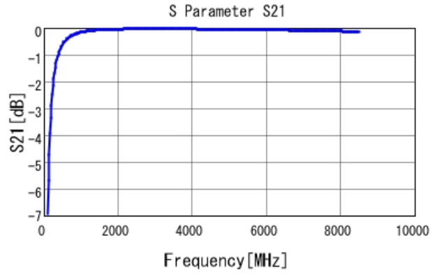
GRM0335C1H8R0WA01 S21 DCOV, 25degC
