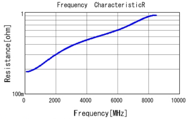
GRM0335C1H8R0WA01 R DCOV, 25degC
