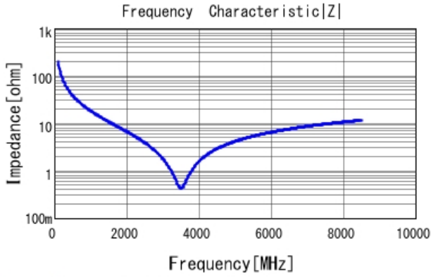
GRM0335C1H8R0WA01 |Z| DCOV, 25degC
