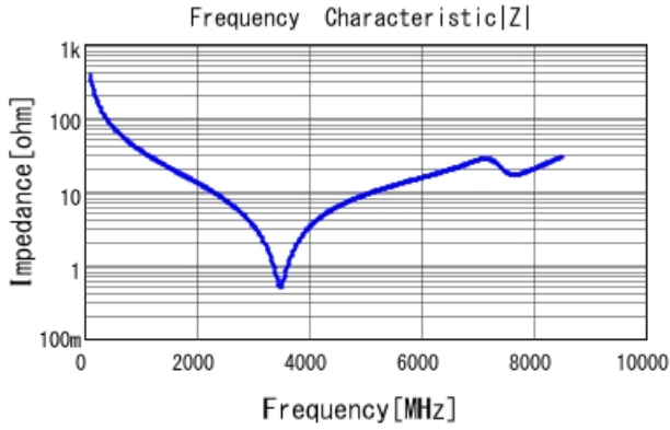
GRM1885C2A4R1CA01 |Z| DCOV, 25degC
