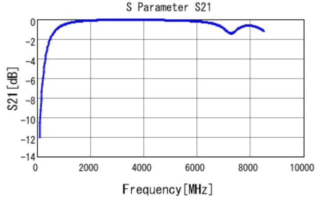
GRM1885C2A4R1CA01 S21 DCOV, 25degC
