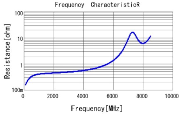
GRM1885C2A4R1CA01 R DCOV, 25degC
