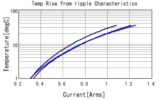
GJM1555C1H180GB01 Temp. rise — 700MHz — 1GHz
