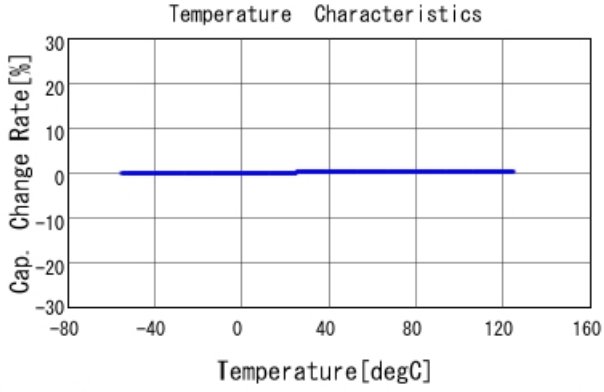
GJM1555C1H180GB01 C-Temp. capchange, DCOV, AC1Vrms
