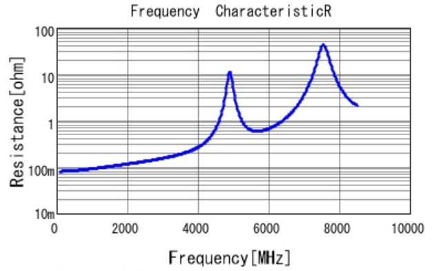
GJM1555C1H180GB01 R DCOV, 25degC
