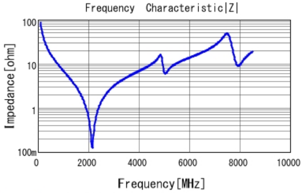
GJM1555C1H180GB01 |Z| DCOV, 25degC
