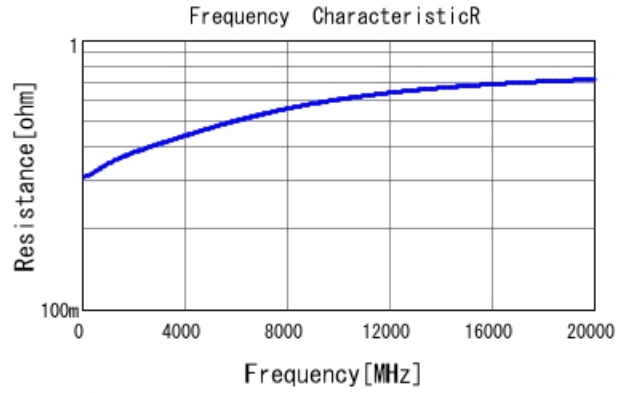
GRM0225C1E1R7WA03 R DCOV, 25degC
