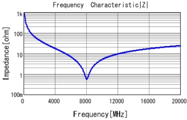
GRM0225C1E1R7WA03 |Z| DCOV, 25degC
