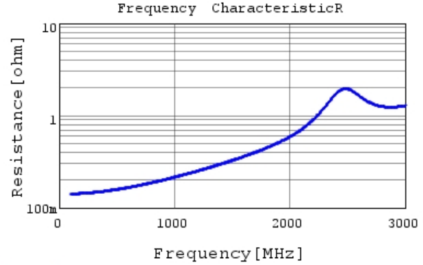
GRM31A5C2J680FW01 R DCOV, 25degC
