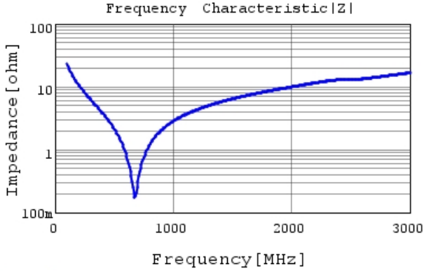
GRM31A5C2J680FW01 |Z| DCOV, 25degC
