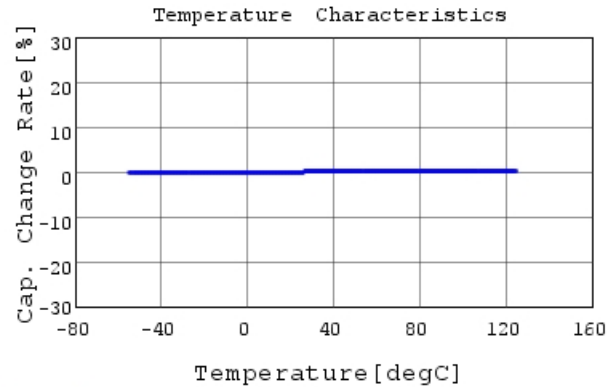
GRM31A5C2J680FW01 C-Temp. capchange, DCOV, 1
