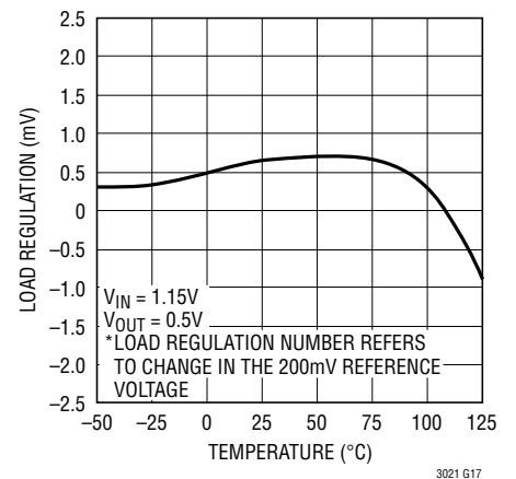
Load Regulation \Delta I_L = 1\text{mA to } 500\text{mA}
