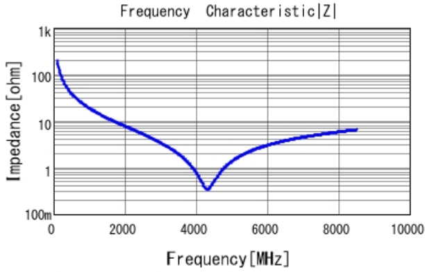
GRM0225C1E8R0WA03 |Z| DCOV, 25degC
