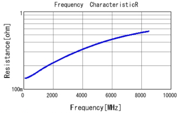
GRM0225C1E8R0WA03 R DCOV, 25degC
