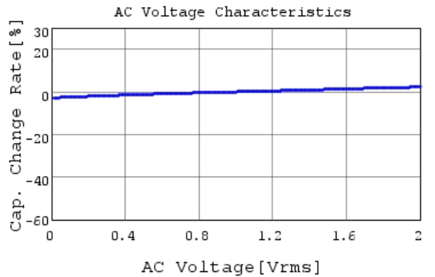
GCJ188R72A104KA01 C-AC Voltage capchange, Dc
