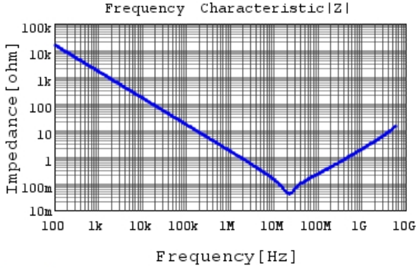
GCJ188R72A104KA01 |Z| DCOV, 25degC
