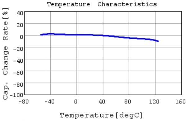
GCJ188R72A104KA01 C-Temp. capchange, DC0.0V,
