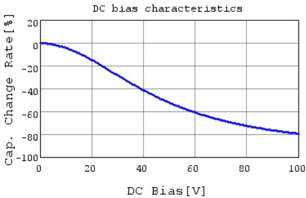
GCJ188R72A104KA01 C-DC bias capchange, 25.0c
