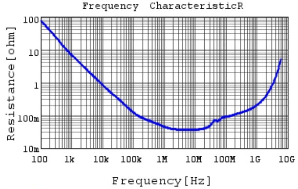
GCJ188R72A104KA01 R DCOV, 25degC
