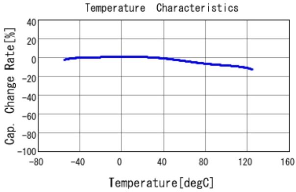
GCJ21BR71E274KA01 C-Temp. capchange, DC0.0V, AC1.C
