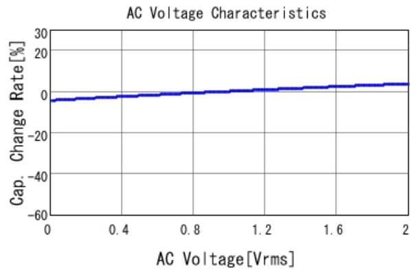
GCJ21BR71E274KA01 C-AC Voltage capchange, DCOV, 25
