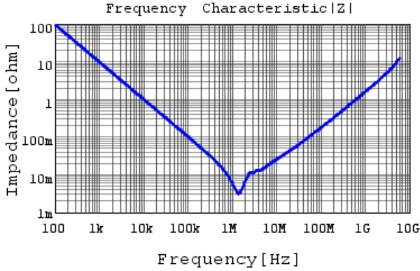
GRM21BR61E226ME44 |Z| DCOV, 25degC
