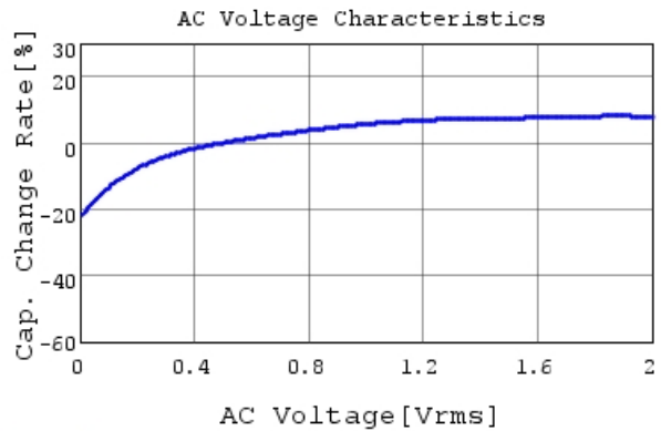
GRM21BR61E226ME44 C-AC Voltage capchange, Dc
