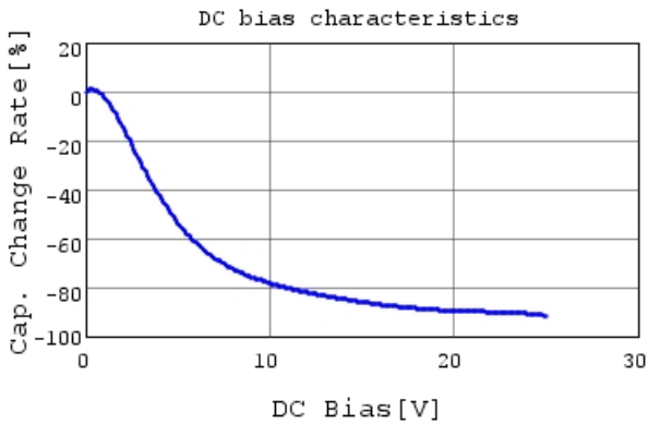
GRM21BR61E226ME44 C-DC bias capchange, 25.0c
