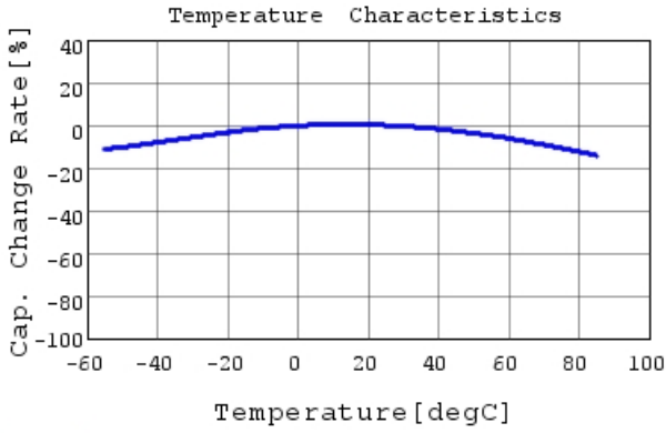
GRM21BR61E226ME44 C-Temp. capchange, DC0.0V,
