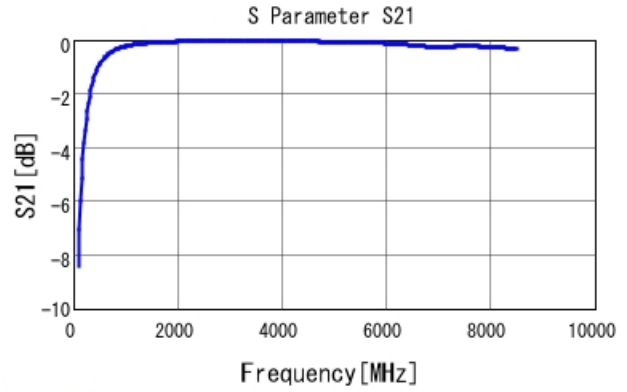
GRM1555C2A6R5CA01 S21 DCOV, 25degC
