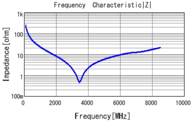
GRM1555C2A6R5CA01 |Z| DCOV, 25degC
