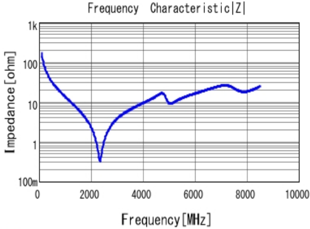
■ GRM1885C1H9R6BA01 |Z| DCOV, 25degC
