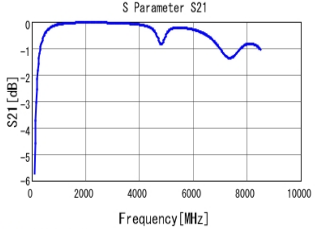
■ GRM1885C1H9R6BA01 S21 DCOV, 25degC
