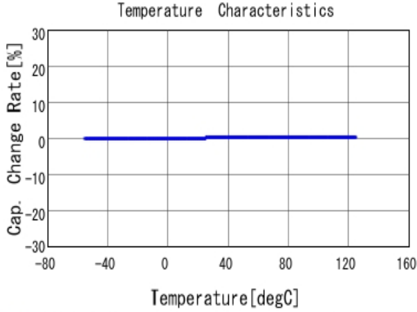
■ GRM1885C1H9R6BA01 C-Temp. capchange, DCOV, AC1Vrms
