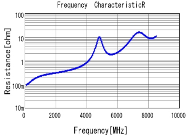
■ GRM1885C1H9R6BA01 R DCOV, 25degC
