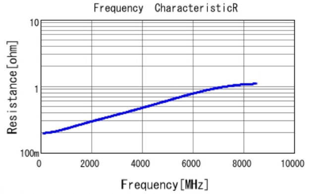
■ GRM0335C2A100JA01 R DCOV, 25degC
