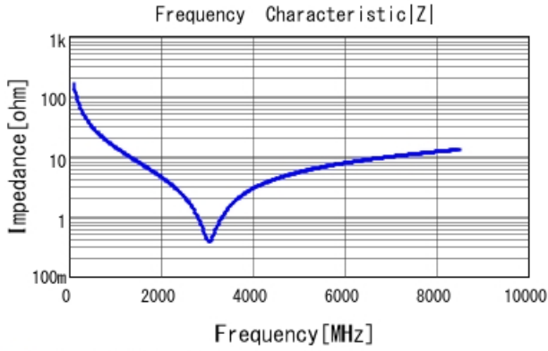
■ GRM0335C2A100JA01 |Z| DCOV, 25degC
