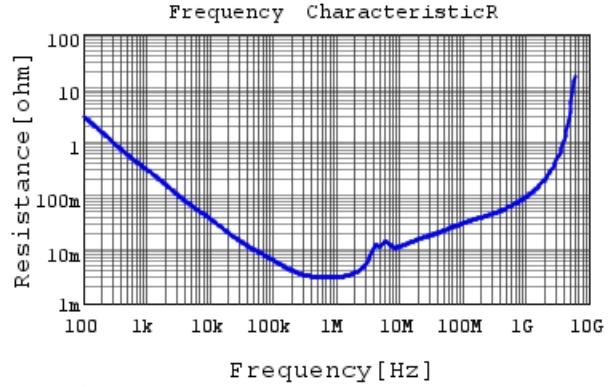
GRM21BZ71C106KE15 R DCOV, 25degC
