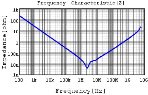
GRM21BZ71C106KE15 |Z| DCOV, 25degC
