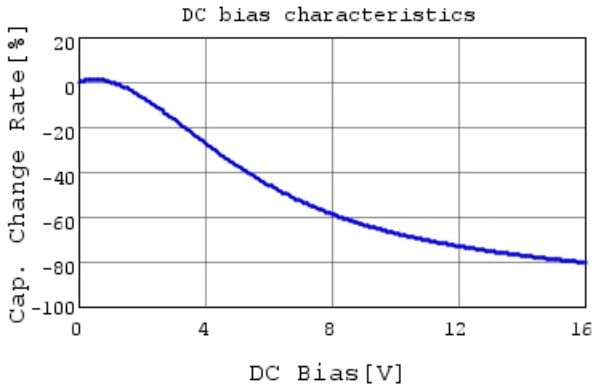
GRM21BZ71C106KE15 C-DC bias capchange, 25.0c
