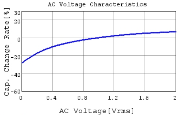
GRM21BZ71C106KE15 C-AC Voltage capchange, Dc
