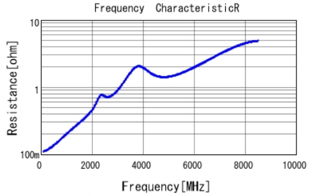
GRM1555C1H750JA01 R DCOV, 25degC
