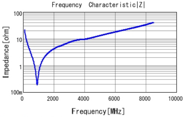
GRM1555C1H750JA01 |Z| DCOV, 25degC
