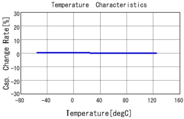
GRM1555C1H750JA01 C-Temp. capchange, DCOV, AC1Vrms
