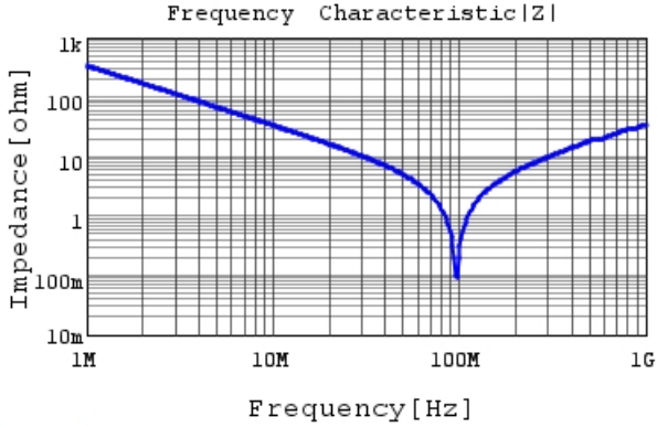
RDE7U3A471J2M1H03A |Z| DCOV, 25degC
