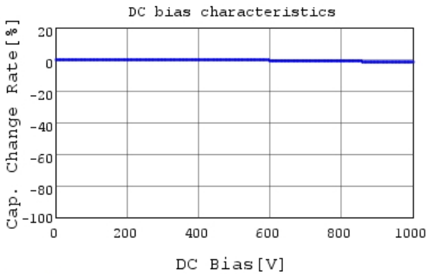
RDE7U3A471J2M1H03A C-DC bias capchange, 25.0
