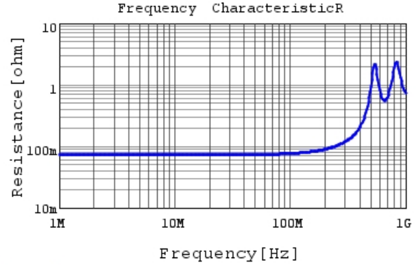
RDE7U3A471J2M1H03A R DCOV, 25degC
