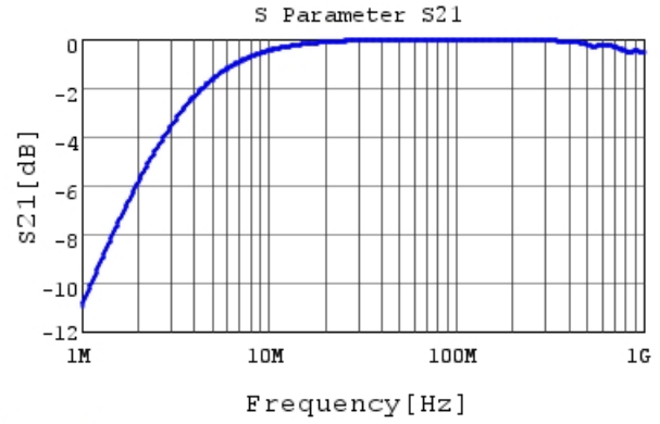
RDE7U3A471J2M1H03A S21 DCOV, 25degC
