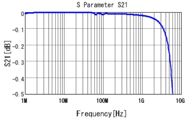
GRM21B7U1H393JA01 S21 DCOV, 25degC
