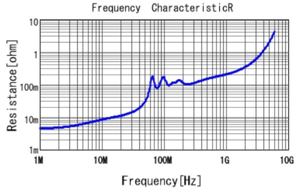
GRM21B7U1H393JA01 R DCOV, 25degC
