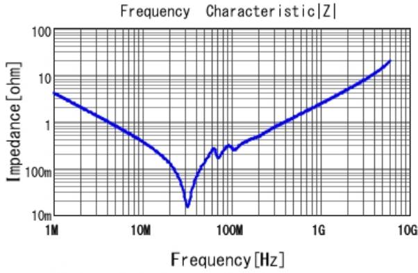
GRM21B7U1H393JA01 |Z| DCOV, 25degC
