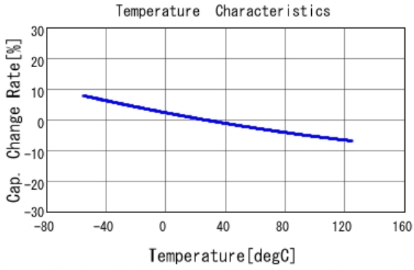
GRM21B7U1H393JA01 C-Temp. capchange, DCOV, AC1Vrms
