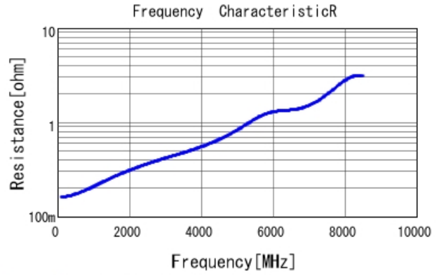
GRM1555C1H9R7WA01 R DCOV, 25degC
