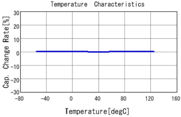
GRM1555C1H9R7WA01 C-Temp. capchange, DCOV, AC1Vrms
