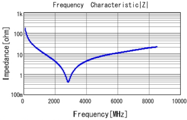
GRM1555C1H9R7WA01 |Z| DCOV, 25degC
