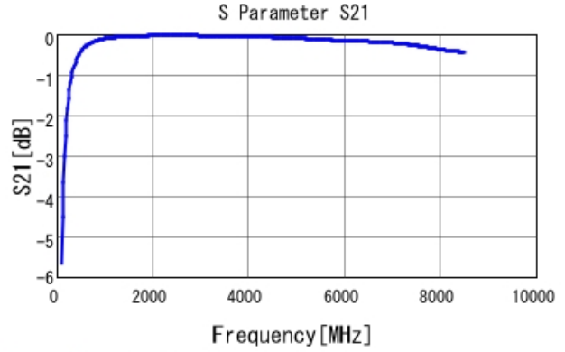
GRM1555C1H9R7WA01 S21 DCOV, 25degC
