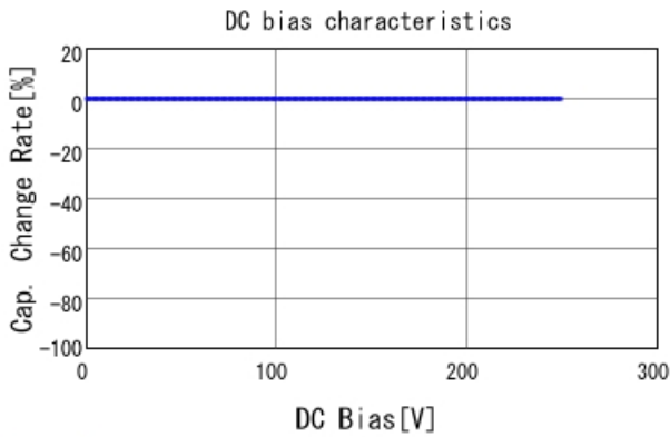
GQM2195G2E1R2CB12 C-DC bias capchange, 25.0degC, A
