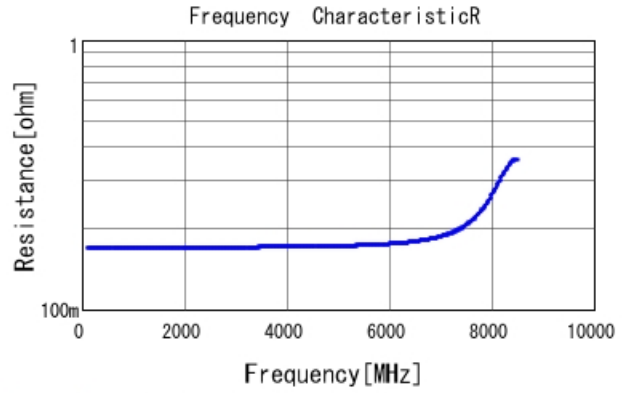
GQM2195G2E1R2CB12 R DCOV, 25degC
