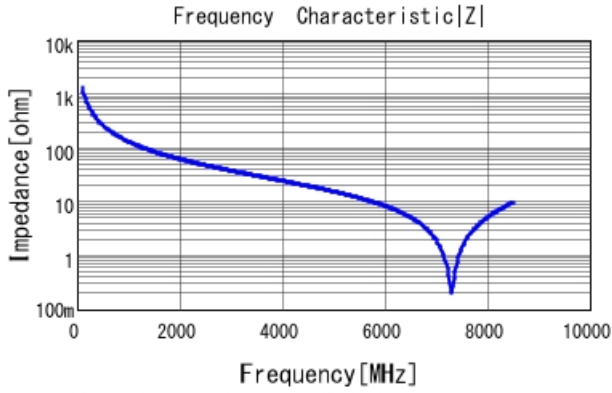
GQM2195G2E1R2CB12 |Z| DCOV, 25degC
