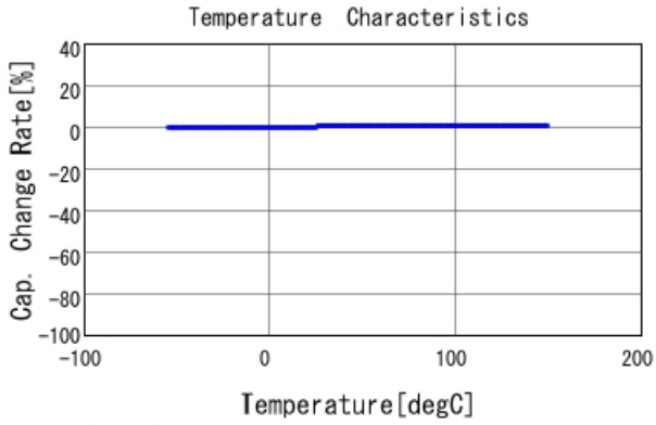
GQM2195G2E1R2CB12 C-Temp. capchange, DCOV, AC1Vrms
