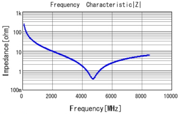
GRM0225C1E6R8WA03 |Z| DCOV, 25degC
