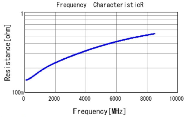
GRM0225C1E6R8WA03 R DCOV, 25degC
