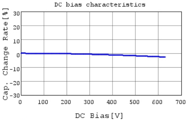
GRM55D7U2J393JW31 C-DC bias capchange, 25.0c
