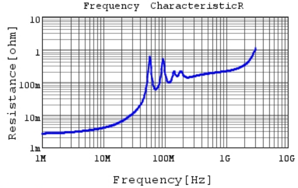
GRM55D7U2J393JW31 R DC0V, 25degC
